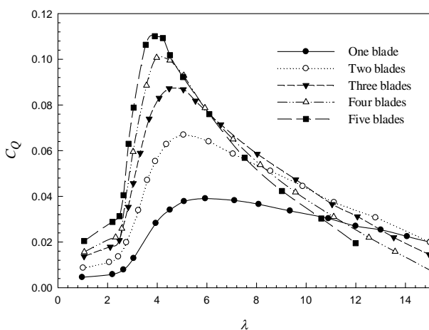
Fig. 2 C_p - \lambda performance curve for wind turbine with different number of blades at \beta = 0^\circ [20]
