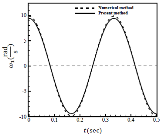
Fig. 10 Angular velocity comparison between present work and Ref [5] of inner wing
