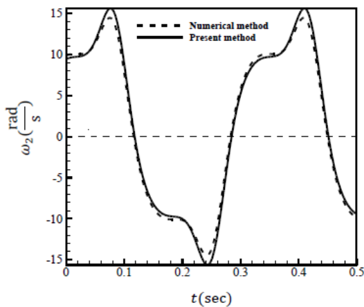
Fig. 9 Angular velocity comparison between present work and of Ref [5] Outer wing
