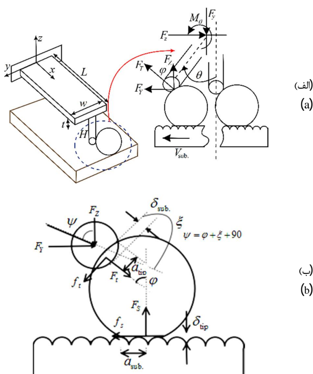
Fig. 3 Displacement of the particle by using the tip of AFM probe, (a) the microcantilever deformation during pushing of the nanoparticle, (b) the interaction forces and deformation of the contact surfaces between the tip/particle and particle/substrate
