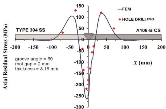
Fig. 7 Axial residual stresses on the outer surface of pipes in the axial direction
