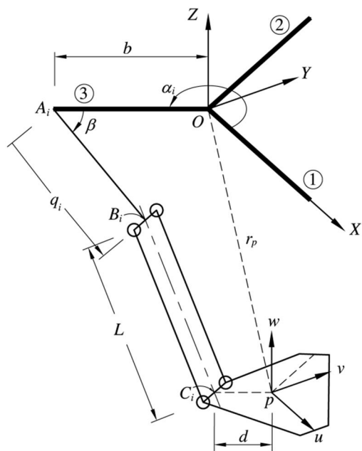
Fig. 4 Schematic of one limb of the 3-[P2(US)] robot
