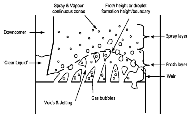
Fig. 19 Clear liquid and froth layer formation on the sieve tray [13]
