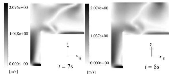
Fig. 13 Liquid velocity distribution in the symmetry plane in different time
