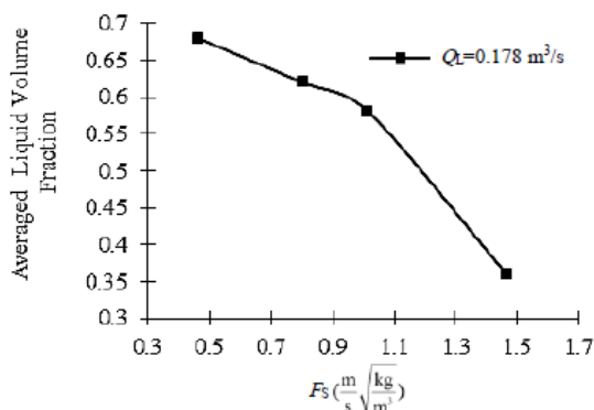
Fig. 21 Averaged liquid volume fraction changes relative to gas flow factor
