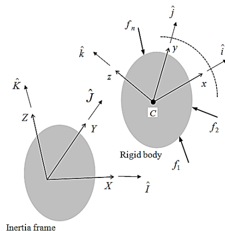
Fig. 6 The force free diagram of the rigid body corresponding to each leg with coordinate systems
