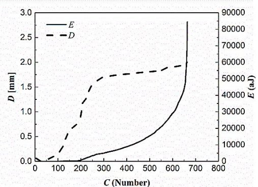
Fig. 7 Diagram of displacement and cumulative energy per cycle for specimen with 0.5 percent carbon nanotube
