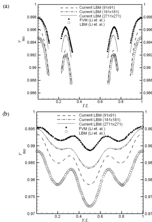
Fig. 7 Profile of isopropanol concentration a- at midline and b- end line of computational domain in compare of Li et al. [5]
