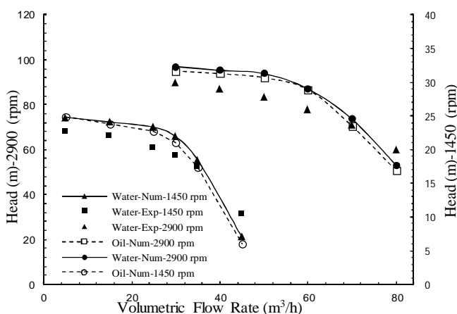
Fig. 6 Numerical and experimental results of Head/h at two angular velocities for water and Crude Oil
