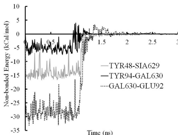
Fig. 9 The variation of non-bonded energies of some interface residues during pulling with constant velocity
