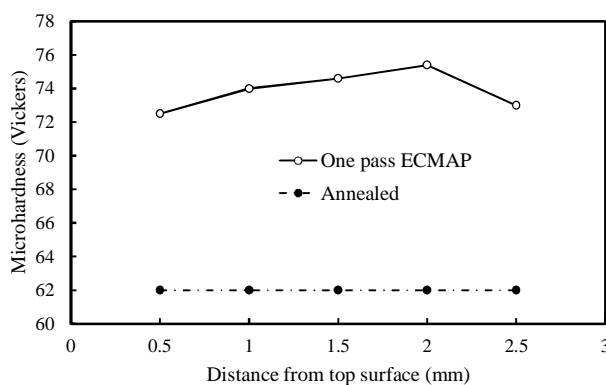
Fig 6 Hardness values for ECMAPed and annealed strips
