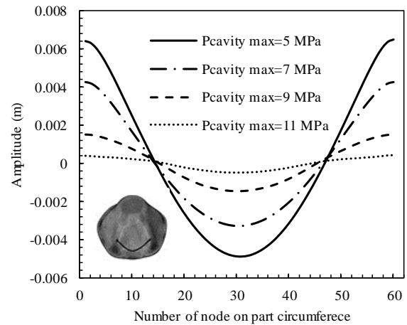
Fig. 22 Effect of cavity pressure on wrinkles, Pradial max=20 MPa
