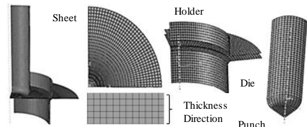
Fig. 2 Finite element model in the assembly with Finite element model of the die set
