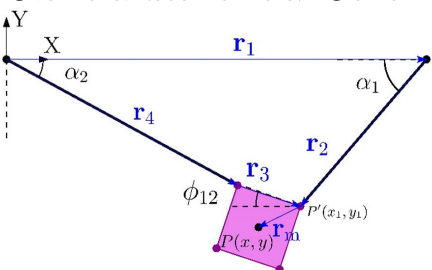
Fig. 3 One side of the CDPR which is assumed as a four-bar linkage
