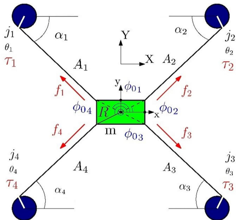
Fig. 2 Schematic view of a planar CDPR with four cables
