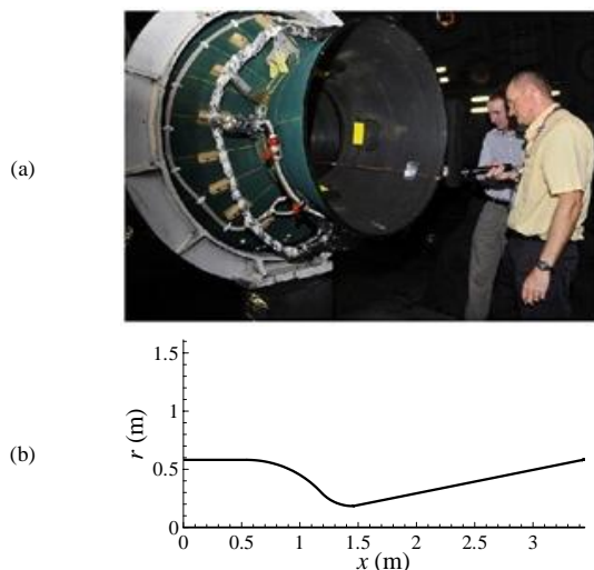
Fig. 3 (a) Minuteman Nozzle and Engine photograph.
