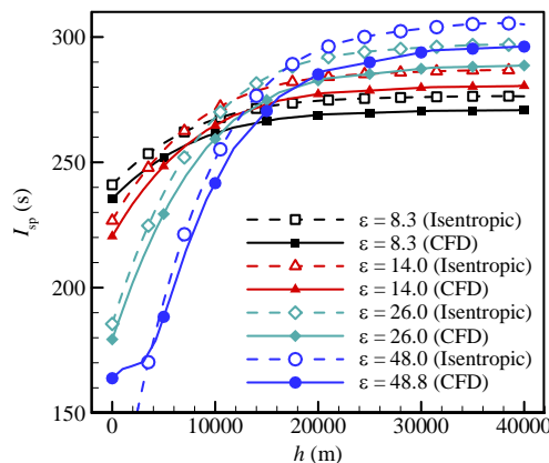
Fig. 11 Numerical and Isentropic Specific Impulse Comparison versus Altitude Change for STAR-27 Specified Expansion Ratios
