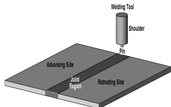
Fig.1 Schematics of friction stir welding process
