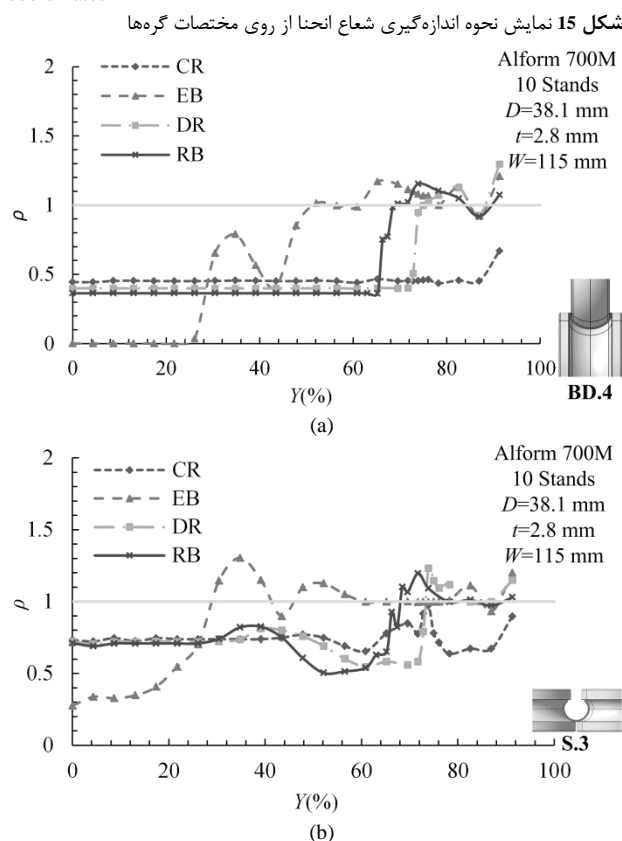
Fig. 16 Distribution of curvature of the cross-section of deformed sheet at the end of (a) breakdown and (b) side stand
