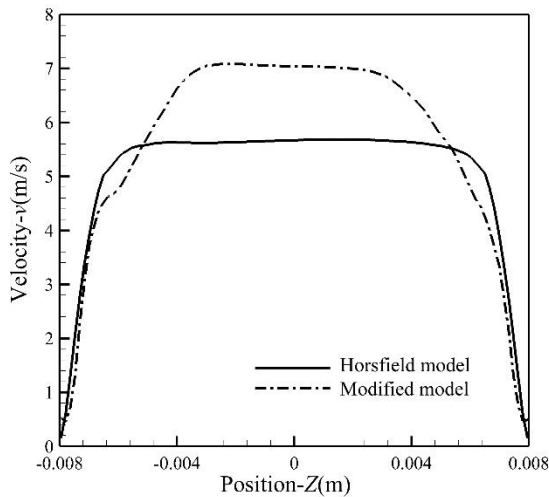
Fig. 21 Velocity profile-line 12 for both of models.
