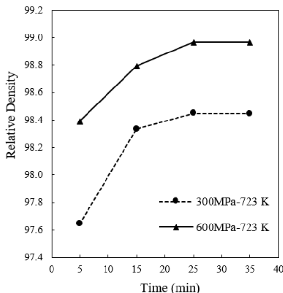
Fig. 2 Relative density variation by time under 300 and 600 MPa compact pressure
