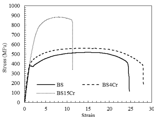
Fig. 11 Effects of Cr addition on Stress-Strain diagrams of weld metals
