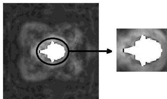
Fig. 9 Asymmetric petaling
