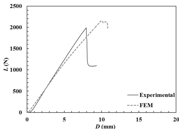
Fig. 19 comparison of numerical and experimental result for square corrugated core
