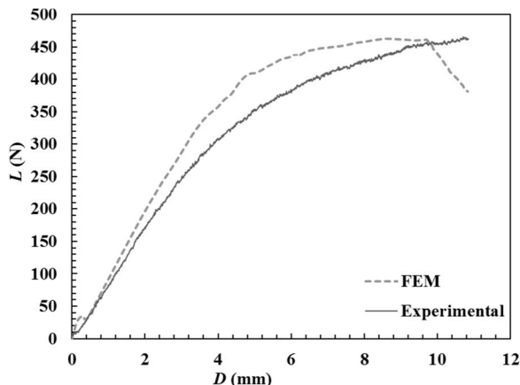
Fig.18 comparison of numerical and experimental result for simple core
