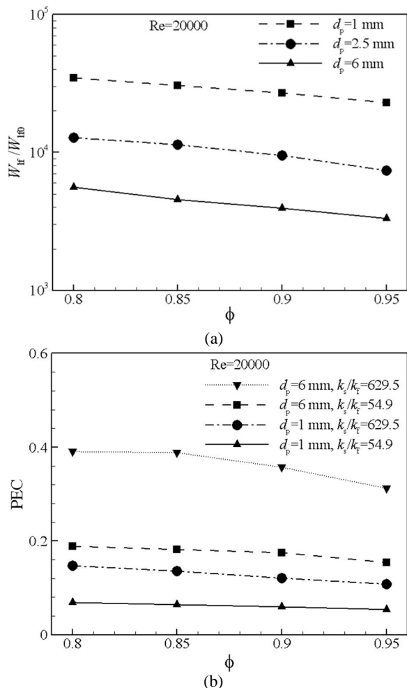
Fig. 13 Investigation of pump lost power (a) and PEC (b) in different property of porous material
