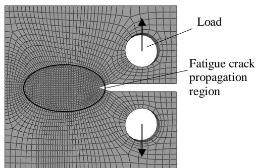
Fig. 3 FE model of meshed CT specimen
