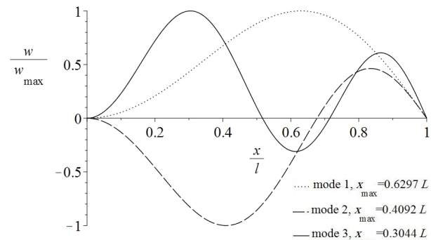
Fig. 9 Buckling deformation for first three modes after replacing supports
