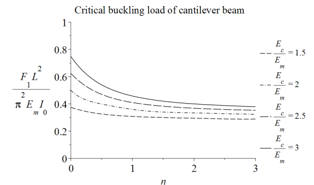
Fig. 6 The influence of material constant and the ratio of the ceramic elasticity modulus to metal elasticity modulus on critical buckling load
