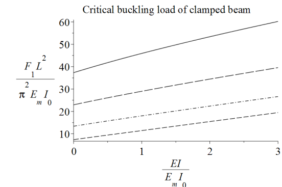
Fig. 5 The influence of flexural rigidity of connecting beam in Hetenyi's model on critical buckling load
