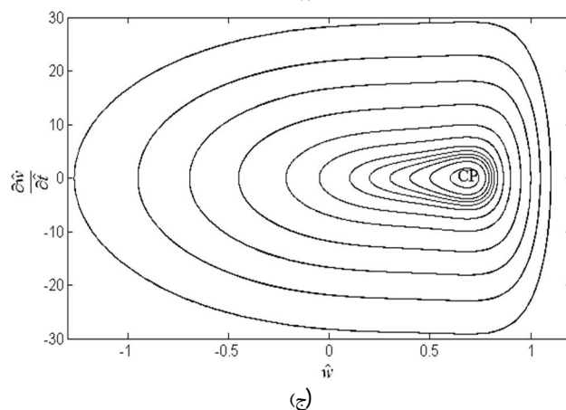
Fig. 4 Phase portraits using first approach for \mu = (0.1L)^2 , a) V = 8V , b) V = 9.4V , c) V = 10V
