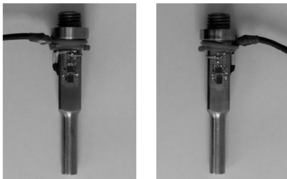
Fig. 11 The strain gages mounted on the impactor
