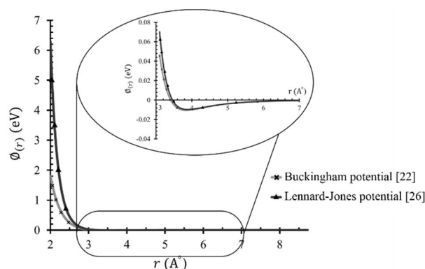
Fig. 1 Potential function behavior versus interatomic distance for Buckingham and Lennard-Jones potential functions [22,26]
