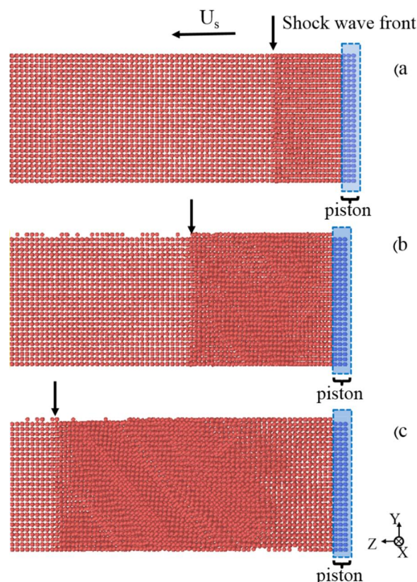
Fig. 2 Snapshots of shockwave propagation (after piston hit) from one side to other side at three different times. a) at time 2ps b) at time 4ps (stop time of piston) c) at time 7ps
