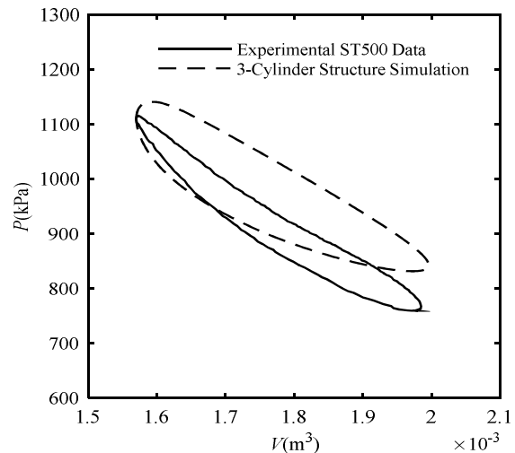
Fig. 9 The P-V diagram of new presented structure model in comparison of experimental data of ST-500 (based on power piston pressure)
