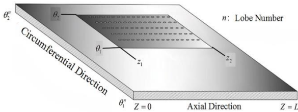
Fig. 3-a Distribution of cylindrical textures in inner surface of journal bearing shell
