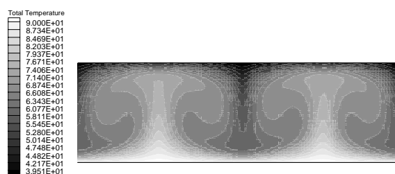
Fig. 3 Temperature contour of the present results
