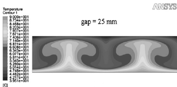
Fig. 2 Temperature contour of Subiantoro and Tiow [3]
