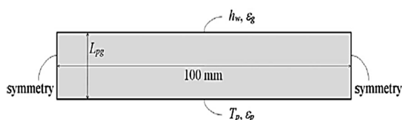
Fig. 1 Rectangular Collector
