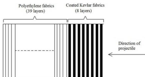
Fig. 11 Schematic image showing how a combination of Kevlar and PE layers is arranged in a panel
