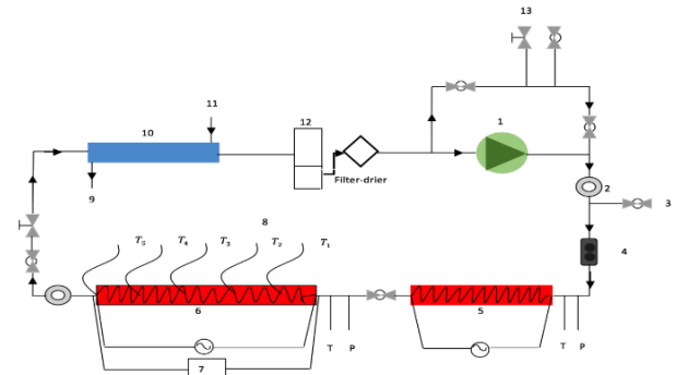
Fig.3 Schematic refrigeration cycle used
