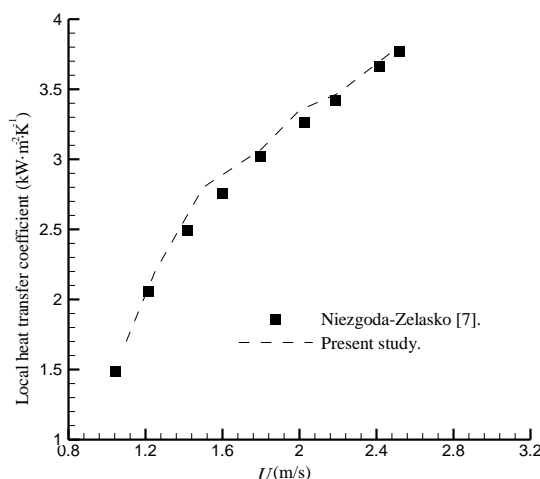
Fig. 5 Comparison of the local heat transfer coefficient in the pipe for different input velocities with numerical results. ( \alpha = 12.8 \text{ wt}\% , d = 0.1 \text{ mm} , D = 16 \text{ mm} , T_{in} = 268.65 \text{ K} , q = 5 \text{ kW/m}^2 )
