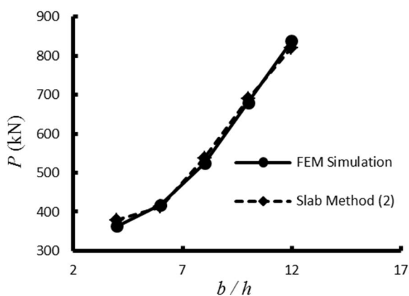
Fig. 8 Compression force with respect to width to thickness ratio
