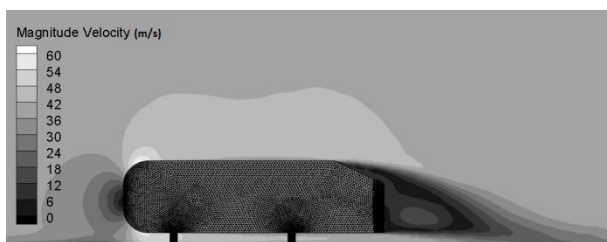
Fig. 2 distribution of velocity with K-\omega-SST model
