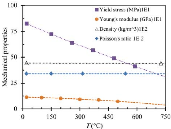
Fig.1 Mechanical properties of titanium alloy (Ti-6Al-4V) at different temperatures [19]
