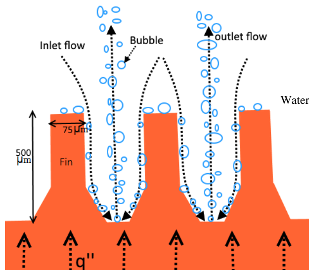
Fig. 14 How flow motion between the fins
