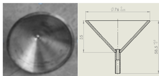
Fig. 1 Copper liner
