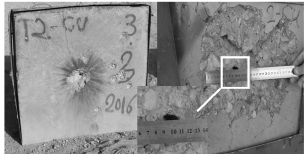
Fig. 8b Second concrete target after forward projectile penetration (Right: back - Left: front)
