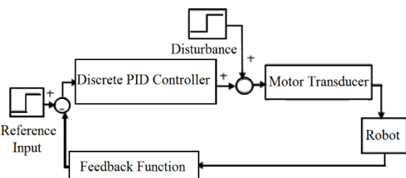
Fig. 2 PID controller simulation
