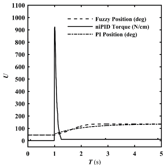
Fig. 15 control signals of different controllers
