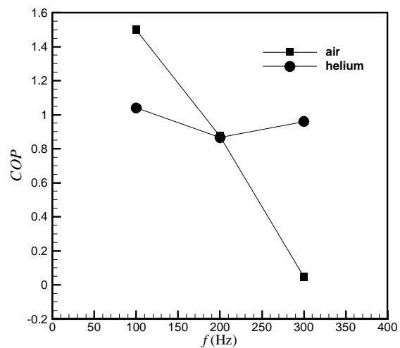
Fig. 12 COP versus frequency, DR=5 , T_c=297 , T_h=300
