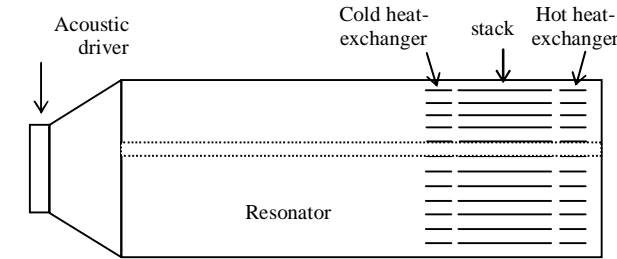
Fig. 1 Geometry of thermoacoustic refrigerator
