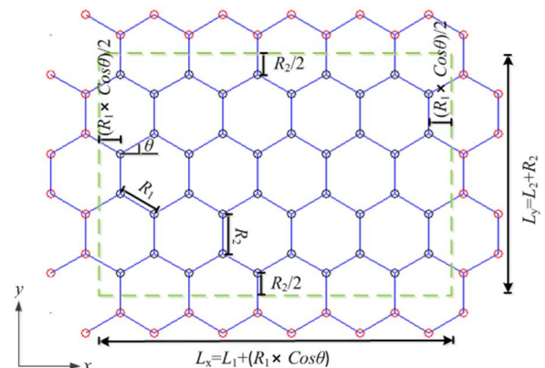
Fig. 9 Imposing Periodic Boundary Conditions in the developed AFEM
