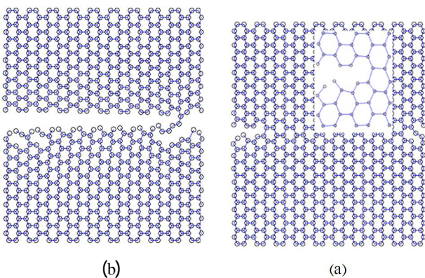
Fig. 6 Failure process of the perfect sample (a) early stages of fracture (b) final configuration
