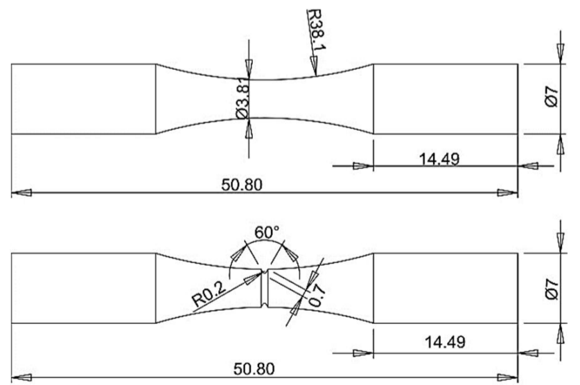
Fig. 3 Plain and V-notched specimen geometry for fatigue test
