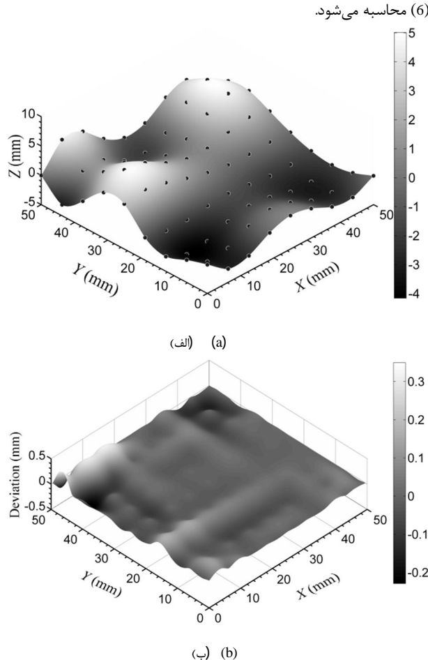
Fig. 4 a) Substitute geometry with sample points (mm), b) deviation from CAD model in uniform sampling strategy in Cartesian space (mm)
