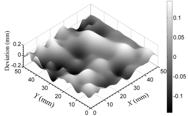
Fig. 9 Substitute geometry deviation from CAD model in sampling strategy by particle swarm algorithm (mm)
