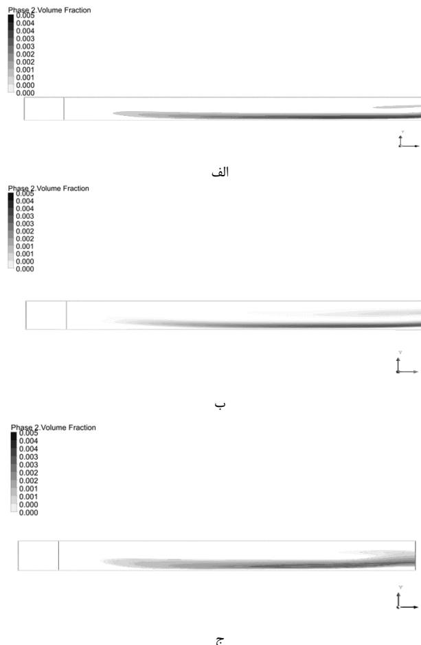
Fig. 8 Contours of volume fraction in the center plane at t = 2.25 S from beginning of the simulation in different grids a) mesh with 42850 grid cells b) mesh with 210547 grid cells c) mesh with 482355 grid cells
