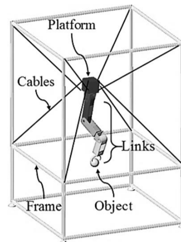
Fig. 1 Structure of the hybrid robot
