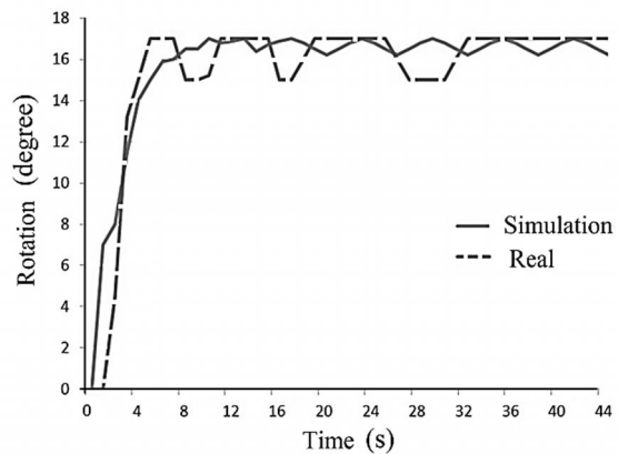
Fig. 11 The rotation angle of the Link 3
