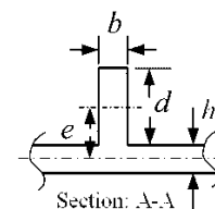
Fig. 3 Geometry of the cross section of the ring support
