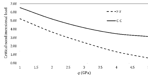
Fig. 9 Effects of variations the lateral pressure on critical buckling pressure for different boundary conditions
