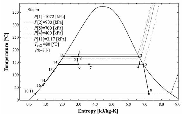
Fig. 5 T-S diagram of the geothermal system
