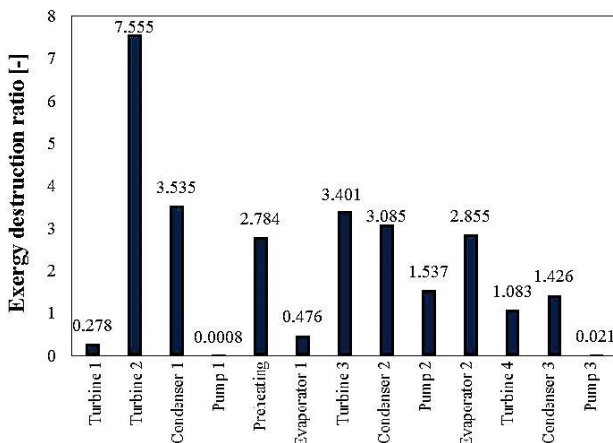
Fig. 19 The rate of exergy destructions in the components of combined cycle with n-butane as a working fluid in comparison to the input exergy
