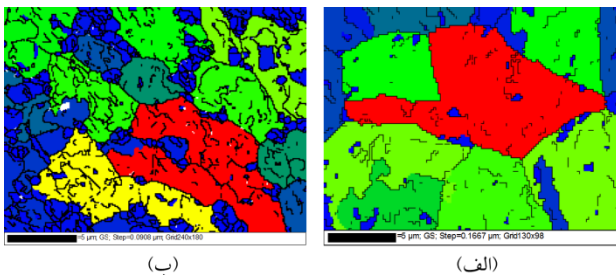
Fig.9 The grains morphology, a-The left side of stir zone, b-The center of stir zone
