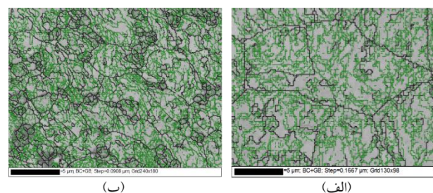
Fig.10 Representation of high-angle boundaries (Mismatch more than 15 degrees indicated with black color) and low-angle boundaries (Mismatch between 2-15 degrees indicated with green color), a- The left side of stir zone, b- the center of stir zone
